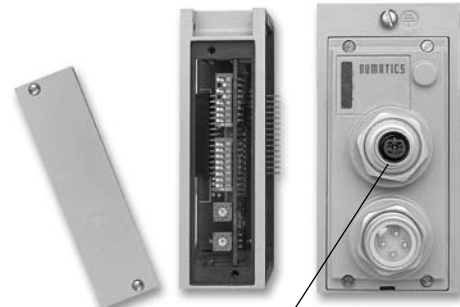
Bus Connector, 5 Pin 12mm Micro Reverse Keyway
